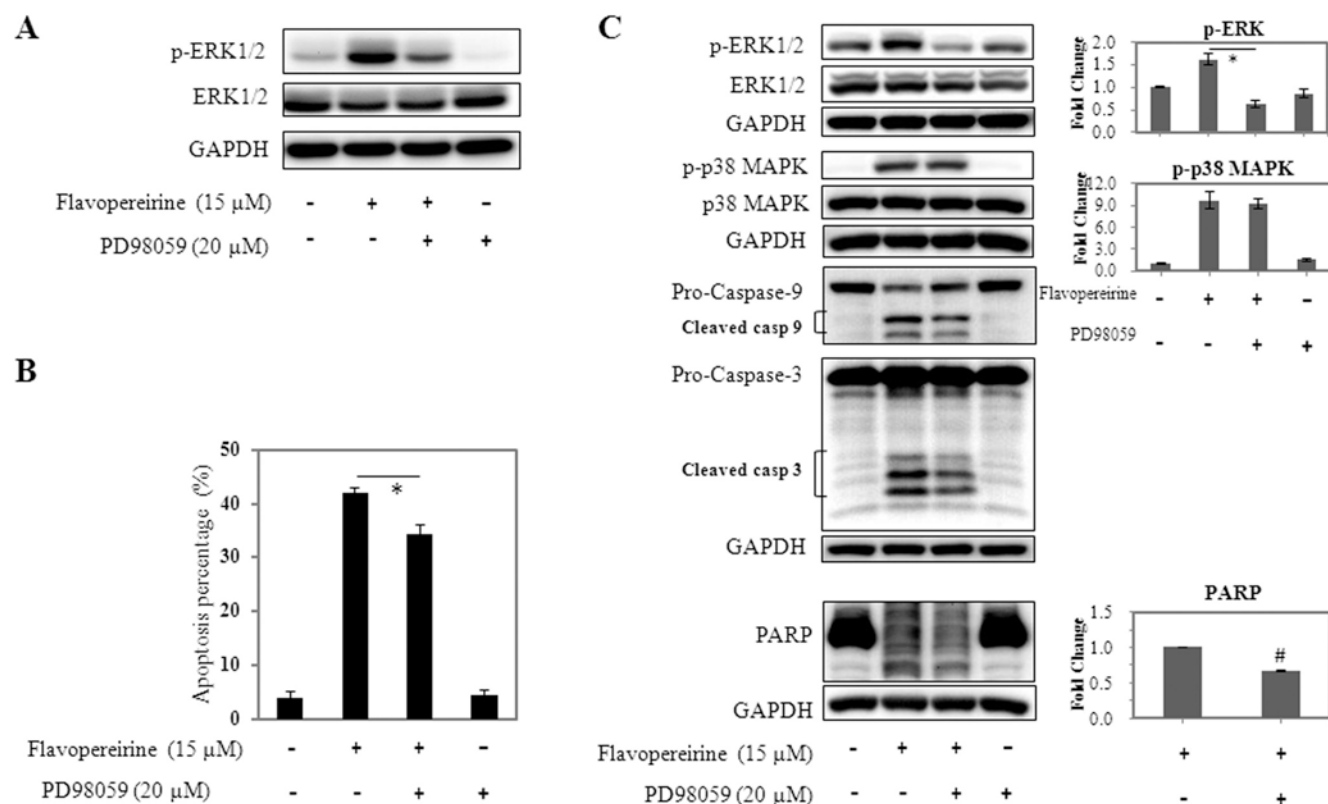
Fig. 5. Determination of the role of ERK in flavopereirine-induced apoptosis. MDA-MB-231 cells were preincubated with the ERK inhibitor PD98059 (20 \mu M) for 2 h and further treated with flavopereirine (15 \mu M) for 48 h. (A) The expression of p-ERK was detected by western blotting. (B) The percentage of apoptotic cells in the presence of flavopereirine with or without PD98059 was examined with Annexin V-FITC and analyzed by flow cytometry. The data were from three individual experiments and are shown in a histogram. (C) The levels of p-ERK, ERK, p-p38 MAPK, p38 MAPK and apoptosis-associated proteins were examined by western blotting. * indicates a significant difference ( P < 0.05 ) between flavopereirine treatment with and without PD98059 treatment as analyzed by one-way ANOVA followed by Bonferroni test. # indicates a significant difference as analyzed by independent t -test.
